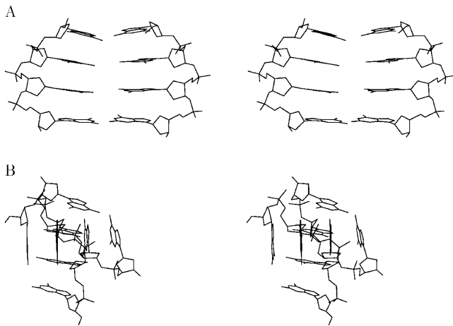
FIGURE 8 Stereo view of the simulated parallel d(\text{GGGG})_2 “diagonal duplex”: (A) starting model; (B) average structure at 3–4 ns of simulation. Only nonhydrogen atoms are depicted.
