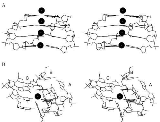
FIGURE 9 Stereo view of the simulated parallel d(\text{GGGG})_3 triplex structure: (A) starting model; (B) average structure at 4–8 ns of simulation. Only nonhydrogen atoms are depicted along with coordinated sodium ions in the molecule center.
