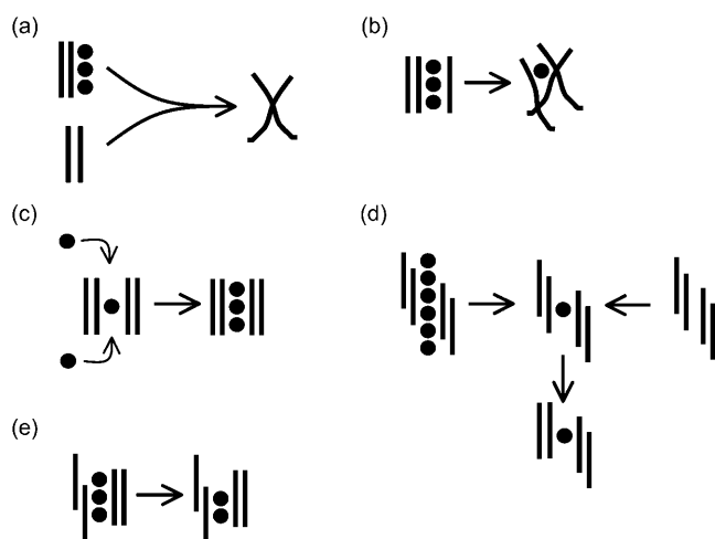
FIGURE 10 Cartoon representation of the simulations performed and structural changes observed in various models on the G-DNA formation pathway. (A) Creation of the “cross-like” dimer from G-DNA parallel- and edge-like duplex models. (B) Creation of the ion-stabilized trimer structure from the G-DNA like triplex model. (C) Spontaneous capture of ions from the solvent by the vacant G-DNA quadruplex. (D) Creation of the single cation stabilized “spiral stem” and spontaneous strand slippage closer to the native quadruplex. (E) Only two ions appear necessary to stabilize the double slipped G-DNA quadruplex model structures.
