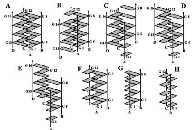
FIGURE 3 Molecular structures of the parallel d(GGGG) 4 stem, G-DNA native, (A), and intermediates studied here: (B) slipped_D_2ions, G-DNA stem with one strand shifted (from Spackova et al. (1999)); (C) shift_AB with A and B strands shifted down and up, respectively; (D) shift_AD with A and D strands shifted down and up respectively; and (E) d(GGGG) 4 as a spiral stem with one central guanine quartet (F) d(GGGG) 3 triplex, (G) parallel d(GGGG) 2 edge duplex (G-DNA dimer_AB), and (H) parallel d(GGGG) 2 diagonal duplex (G-DNA dimer_AC). See text for further details.
