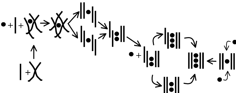
FIGURE 11 Cartoon representation of a possible folding pathway as suggested by the simulations. The key intermediates are the following: 1), cross-like hydrogen-bonded duplexes that do not interact with ions and that possess free base hydrogen bonds capable of intercepting additional strands; 2), cross-like hydrogen-bonded triplexes that are modestly stabilized by a cation and still possess free base hydrogen bonds to intercept additional strands; and 3), a wide range of stable four-stranded intermediates with structured quartets stabilized by monovalent cations.
