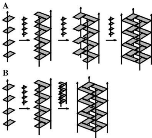
FIGURE 2 Two predominant hypothetical models proposed for G-DNA formation from experiments (Hardin et al., 1991): (A) stepwise strand addition and (B) duplex dimerization.
