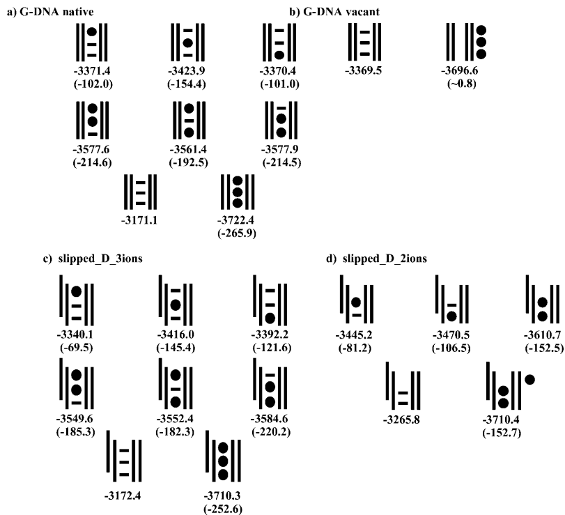
FIGURE 12 Schematic representation of the free energy of individual ion binding sites extracted from four-stranded d(\text{GGGG})_4 model trajectories: native and vacant stem, and single-slipped stems with two or three cations. Solid balls inside the double vertical lines (representing the DNA structure where the 5' end is up) represent bound ions whereas those outside the DNA are free but associated ions (those closest to and outside the channel). Horizontal lines represent empty ion positions in the various models. Below each schematic model is the total free energy of the d(\text{GGGG})_4 model including the ions shown by solid balls, and in parentheses is the (total) ion-DNA interaction energy (defined as the absolute free energy of the d(\text{GGGG})_4 -ion complex minus the free energies of the d(\text{GGGG})_4 model and ions calculated separately). All the free energies are in kcal/mol. Solute entropic components are not included. Note that for a reasonable comparison of the absolute free energies, the same number of explicit cations must be included into the analysis.
