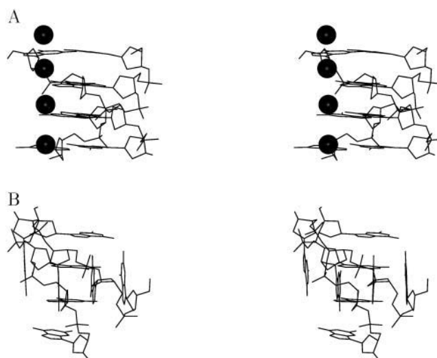
FIGURE 7 Stereo representation of the simulated parallel d(GGGG) 2 “edge duplex”: (A) starting model; (B) average structure (last ns). Only nonhydrogen atoms are depicted along with coordinated sodium ions.
