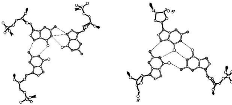
FIGURE 5 View of the triad bases from the two ends of the shift_AB structure, including a representation of the hydrogen bonding between the bases. The triad geometry is regulated by the position of the cations stabilizing the adjacent quartet region.
