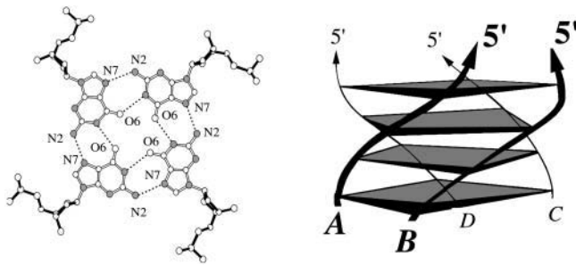
FIGURE 1 Schematic drawing of a guanine quadruplex stem formed by d(GGGG)_4 . This structure is stabilized by four stacked guanine quartet layers (left) and has all strands oriented in parallel (arrows) (right) with all anti glycosidic bonds.
