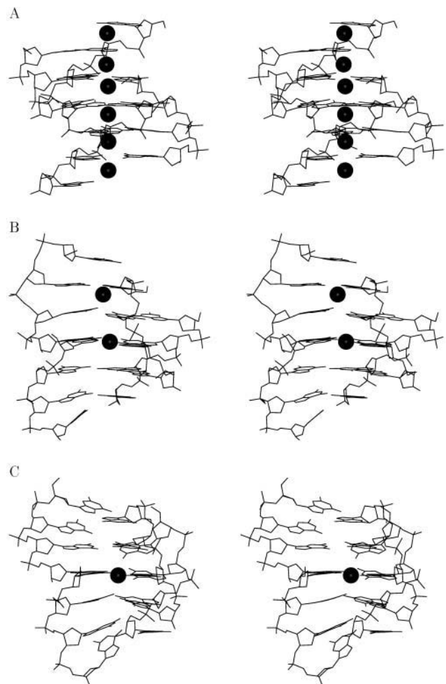
FIGURE 6 Line drawing stereo representation of the simulated “spiral stem” structure: ( A ) starting model, ( B ) average structure at 7–9 ns, and ( C ) average structure at 10–11 ns of simulation. Only nonhydrogen atoms are depicted along with coordinated sodium ions along the helical axis of the four-stranded molecule (molecules are not shown in the same side view).
