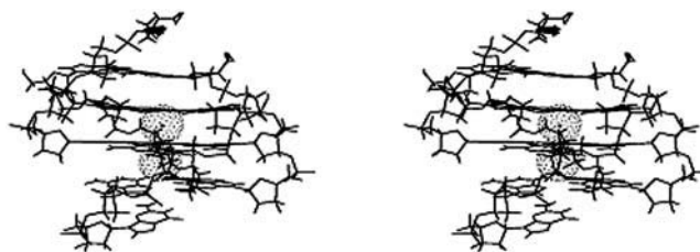
FIGURE 4 Stereo view of the 2–5 ns average structure from the shift_AB simulation.
